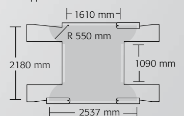
Supported area of the swivel arms
