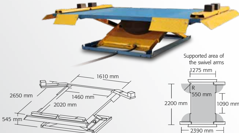
With the cross beam (page 13) the lifting points of large vehicles are ensured.
