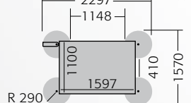
Supported area of the swivel arms in mm HM 1100-04
