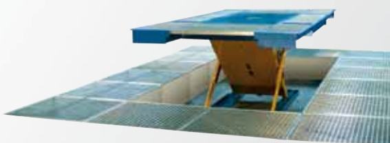
The HLS1600-U immersed for the work on the upper parts of the vehicle.
