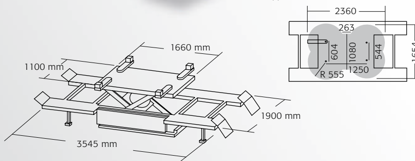
Supported area of the swivel arms in mm
