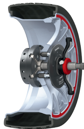
The correct use of the QuickPlate on a wheel (in connection with QuickHub and SoftGrip)
